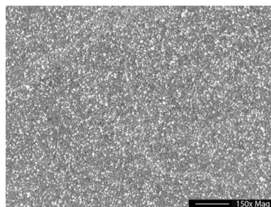
The open porosity of graphite (top) is key to the impregnation process. Copper graphite is formed when copper fills the pores (bottom)
