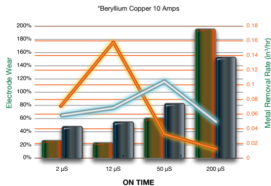
Chart 3 Effects of On Time Performance for Thermally Conductive Materials
