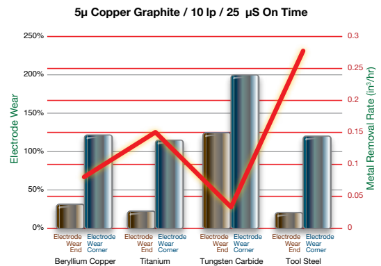
Chart 2 Effects of Conductivity on EDM Performance
